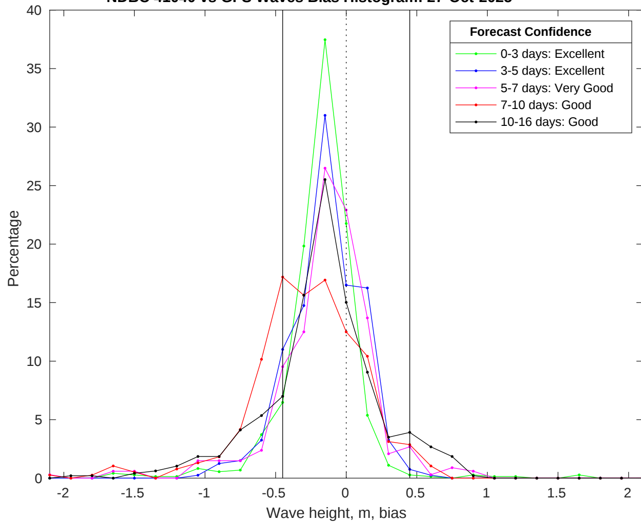
NDBC 41040 vs GFS Waves Bias Histogram: 27-Oct-2025
