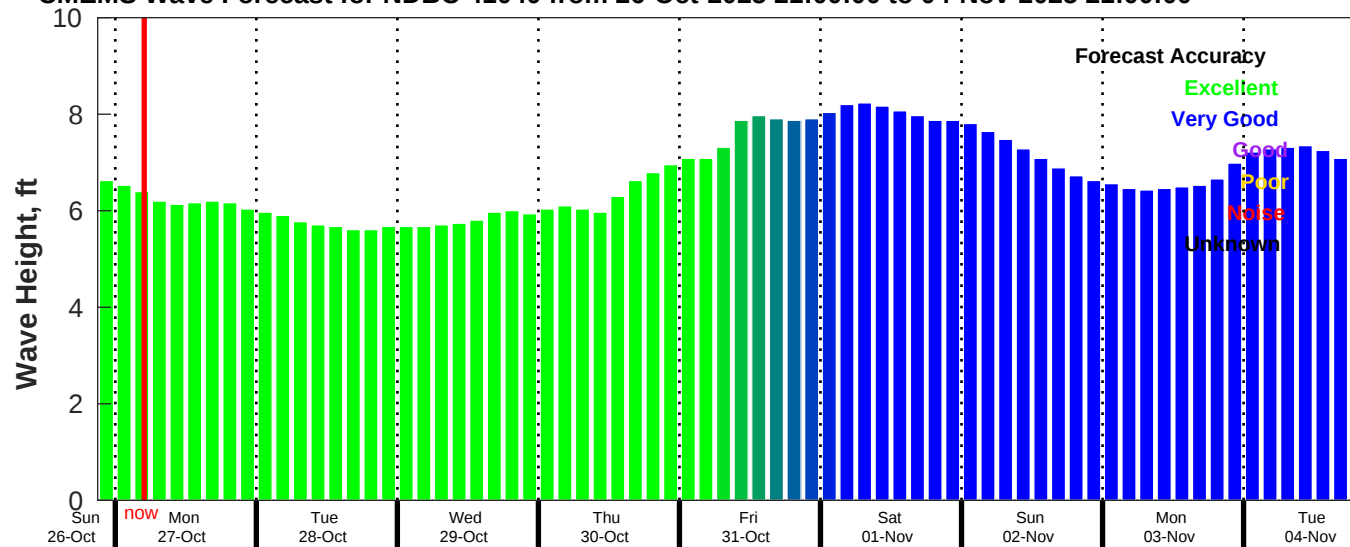
CMEMS Wave Forecast for NDBC 41040 from 26-Oct-2025 21:00:00 to 04-Nov-2025 21:00:00
