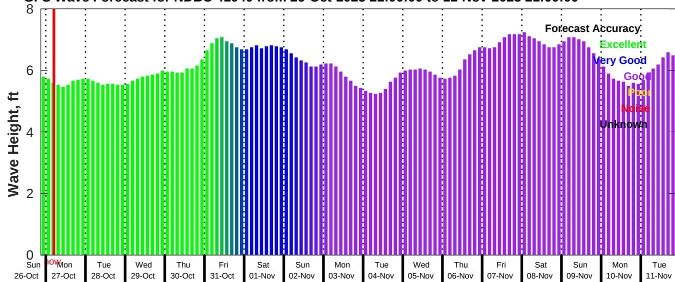
GFS Wave Forecast for NDBC 41040 from 26-Oct-2025 21:00:00 to 11-Nov-2025 21:00:00
