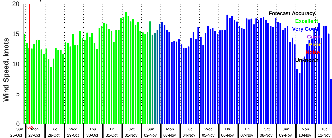
GFS Wind Speed Forecast for NDBC 41040 from 26-Oct-2025 21:00:00 to 11-Nov-2025 21:00:00
