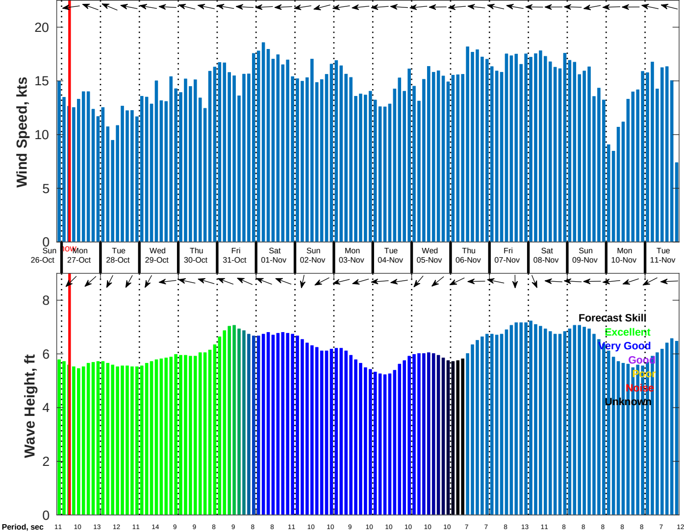
Wind & Wave Forecast for NDBC 41040 from 26-Oct-2025 21:00:00 to 11-Nov-2025 21:00:00
