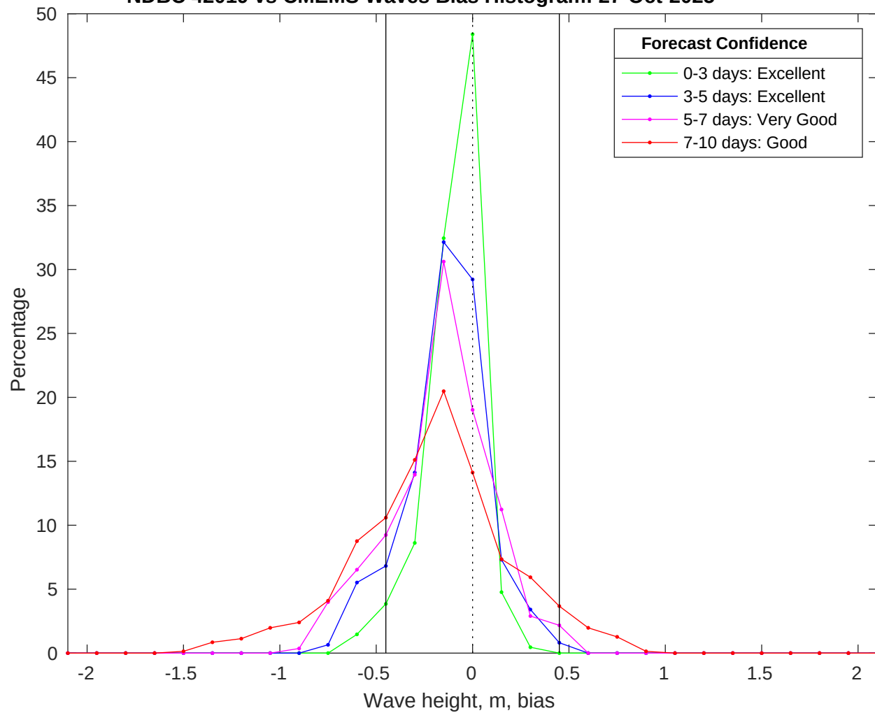
NDBC 42019 vs CMEMS Waves Bias Histogram: 27-Oct-2025
