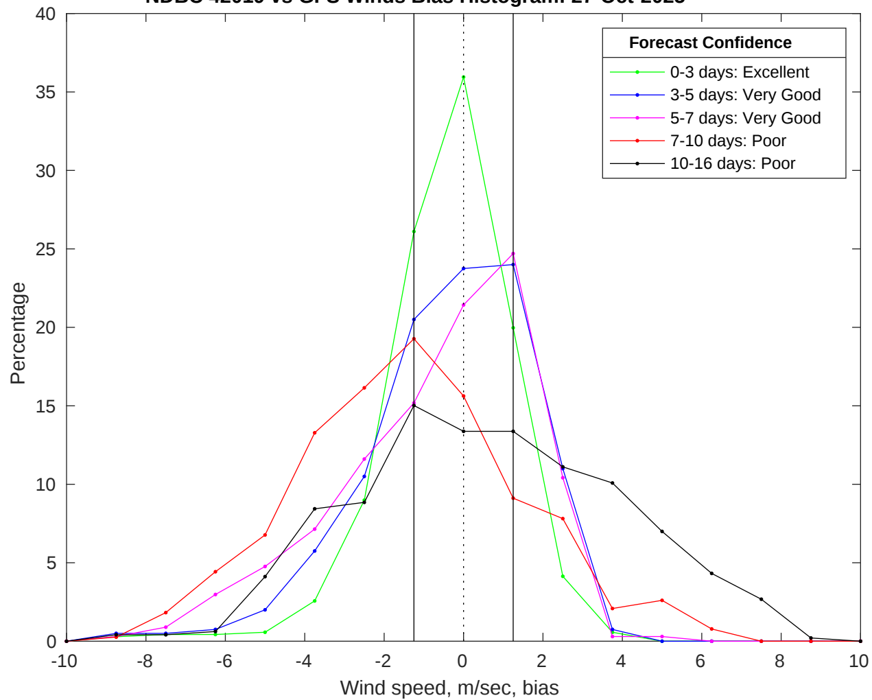
NDBC 42019 vs GFS Winds Bias Histogram: 27-Oct-2025
