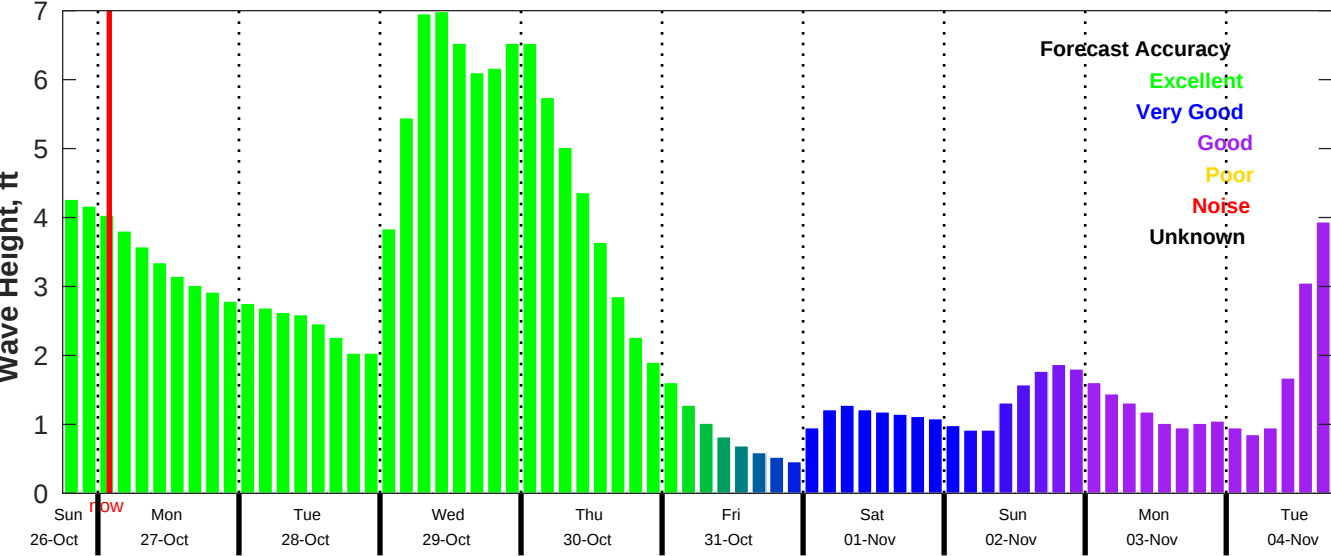
CMEMS Wave Forecast for NDBC 42019 from 26-Oct-2025 18:00:00 to 04-Nov-2025 18:00:00
