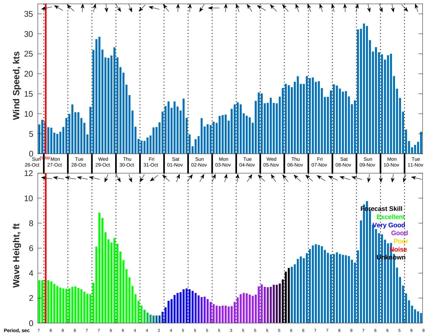
Wind & Wave Forecast for NDBC 42019 from 26-Oct-2025 18:00:00 to 11-Nov-2025 18:00:00
