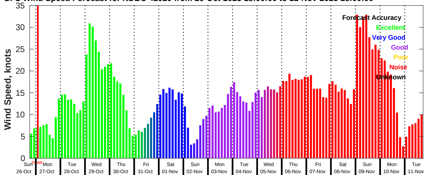
GFS Wind Speed Forecast for NDBC 42020 from 26-Oct-2025 18:00:00 to 11-Nov-2025 18:00:00
