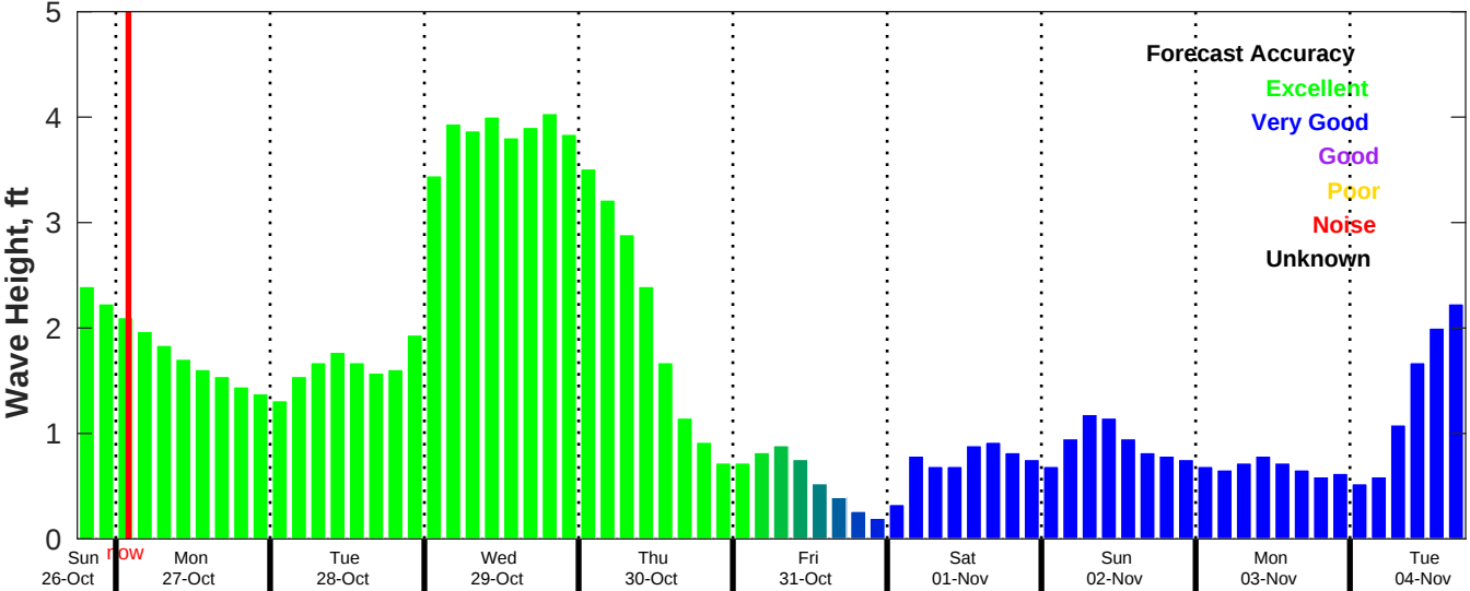
CMEMS Wave Forecast for NDBC 42035 from 26-Oct-2025 18:00:00 to 04-Nov-2025 18:00:00
