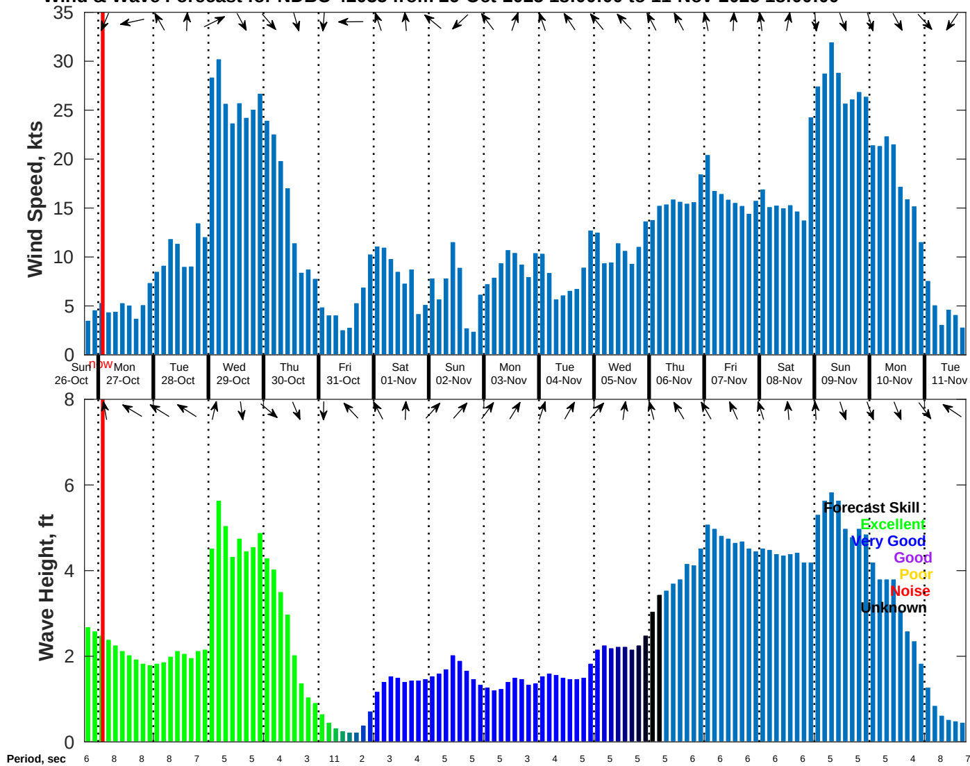
Wind & Wave Forecast for NDBC 42035 from 26-Oct-2025 18:00:00 to 11-Nov-2025 18:00:00
