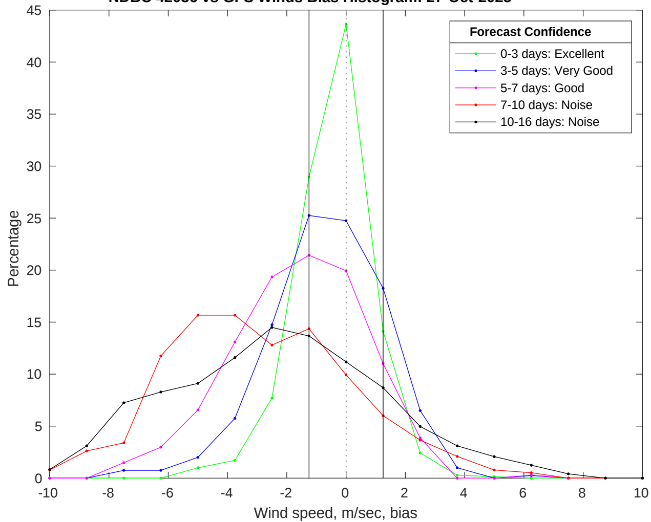
NDBC 42036 vs GFS Winds Bias Histogram: 27-Oct-2025
