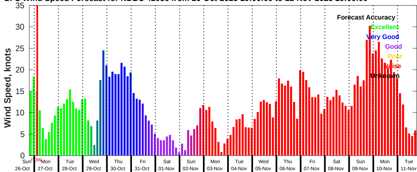
GFS Wind Speed Forecast for NDBC 42036 from 26-Oct-2025 19:00:00 to 11-Nov-2025 19:00:00
