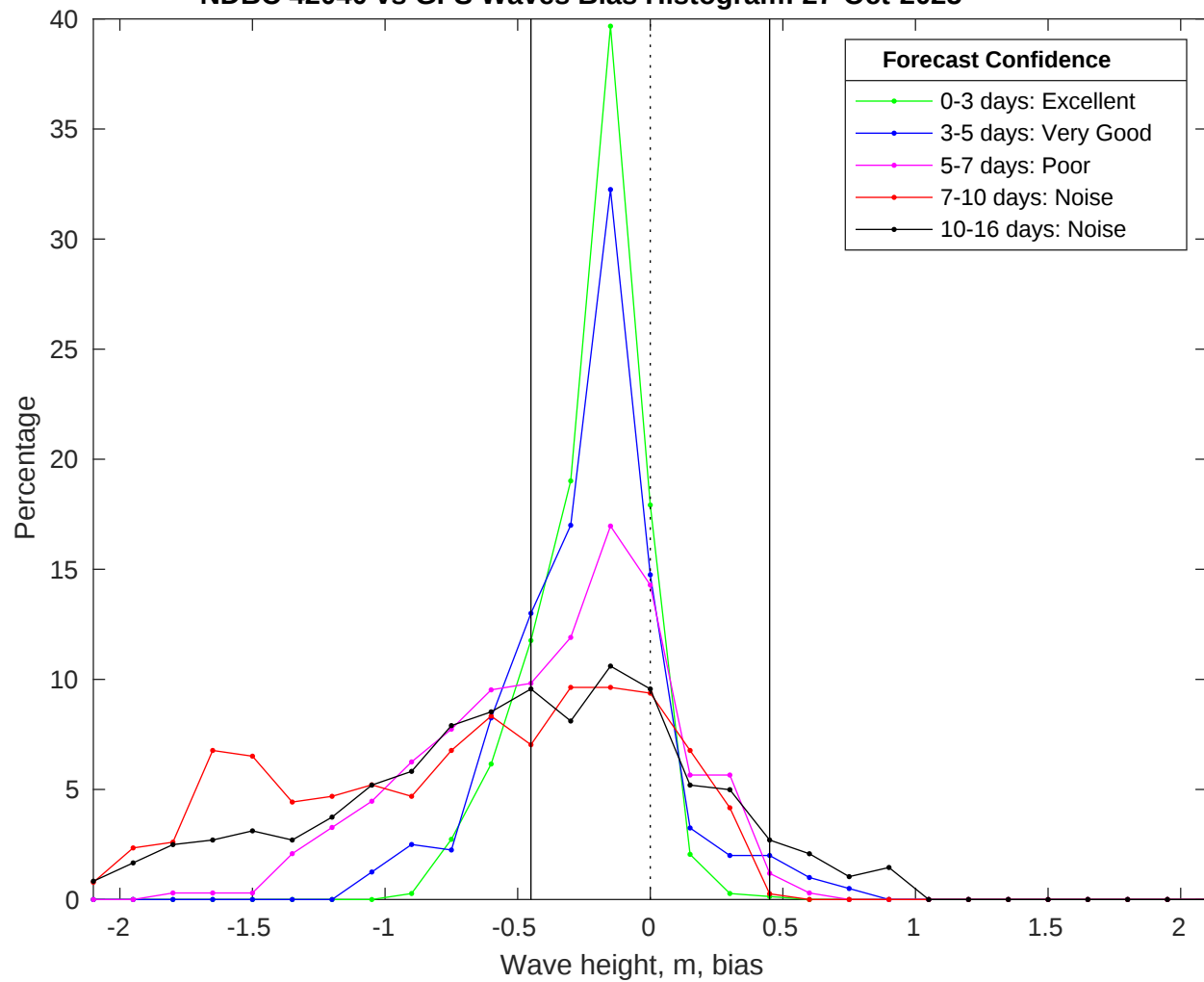
NDBC 42040 vs GFS Waves Bias Histogram: 27-Oct-2025
