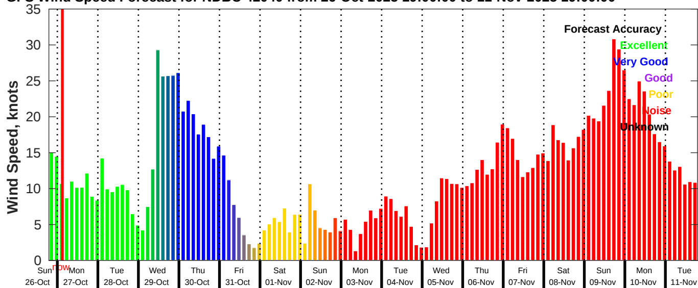
GFS Wind Speed Forecast for NDBC 42040 from 26-Oct-2025 19:00:00 to 11-Nov-2025 19:00:00
