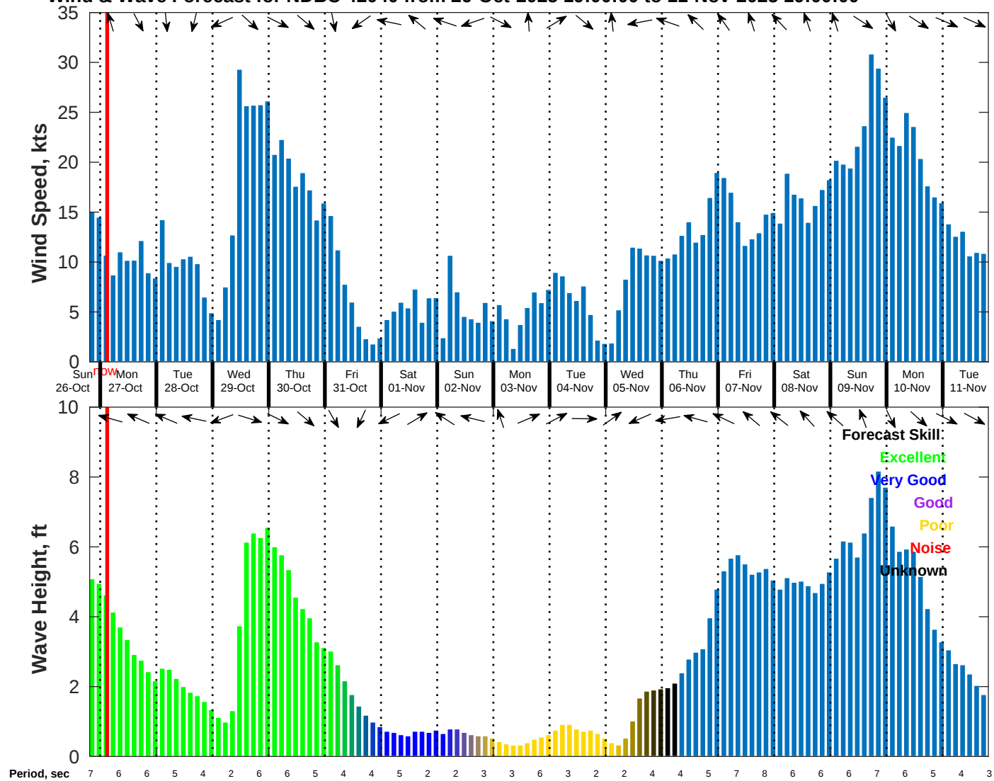
Wind & Wave Forecast for NDBC 42040 from 26-Oct-2025 19:00:00 to 11-Nov-2025 19:00:00
