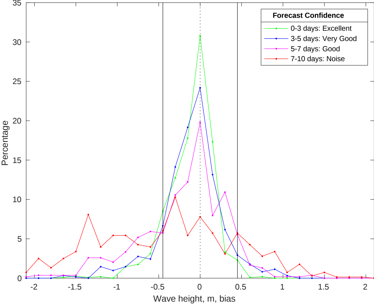
NDBC 44008 vs CMEMS Waves Bias Histogram: 27-Oct-2025
