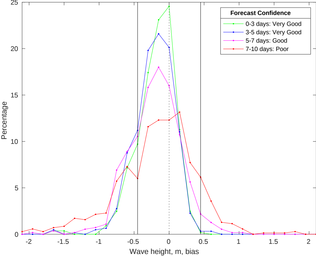
NDBC 46011 vs CMEMS Waves Bias Histogram: 27-Oct-2025
