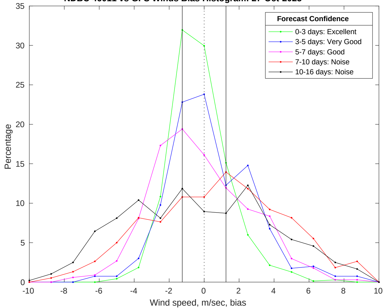
NDBC 46011 vs GFS Winds Bias Histogram: 27-Oct-2025
