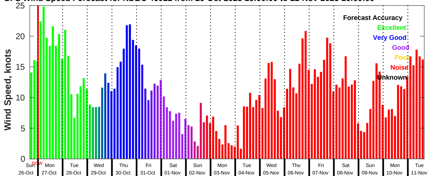
GFS Wind Speed Forecast for NDBC 46011 from 26-Oct-2025 16:00:00 to 11-Nov-2025 16:00:00
