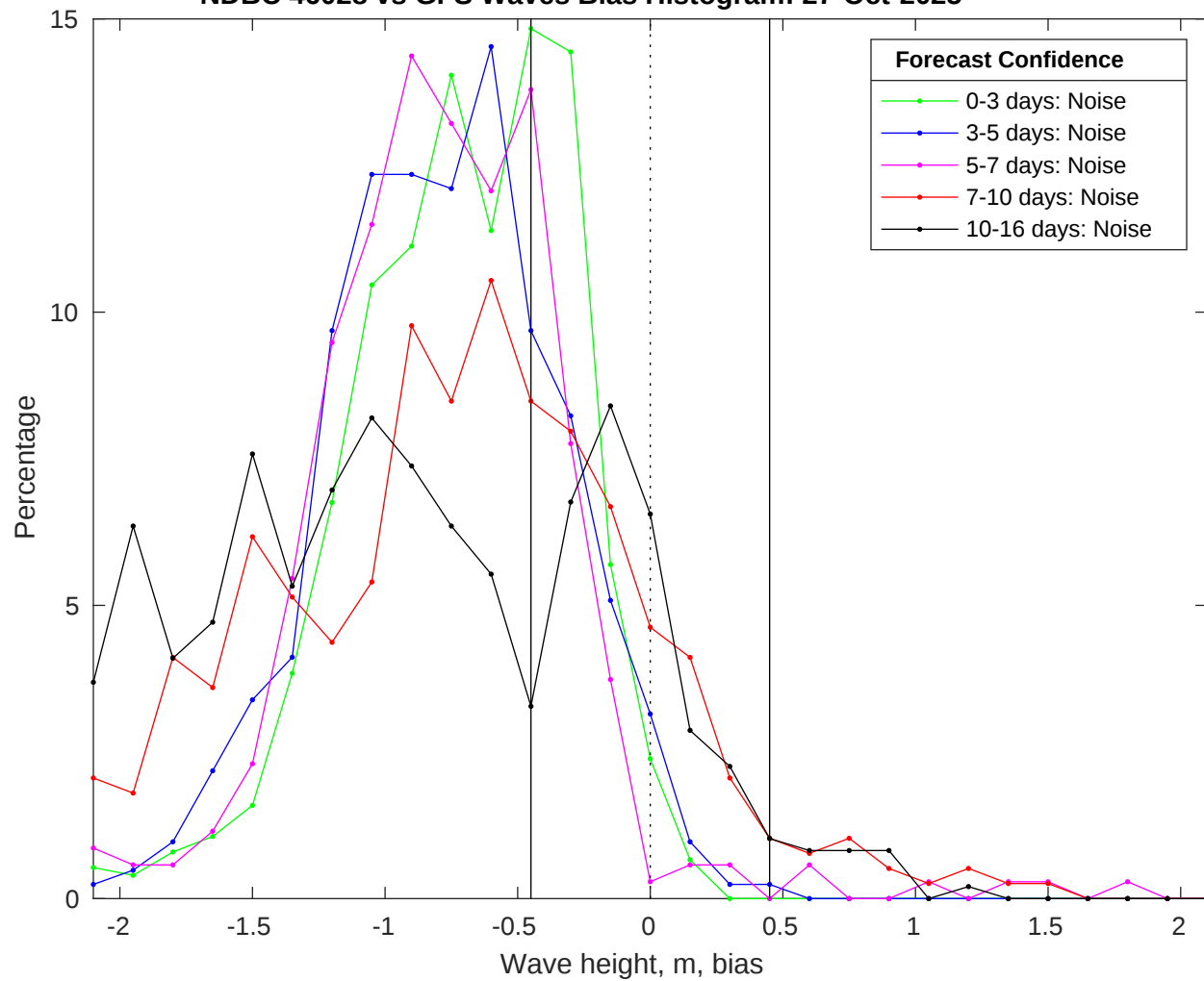
NDBC 46028 vs GFS Waves Bias Histogram: 27-Oct-2025
