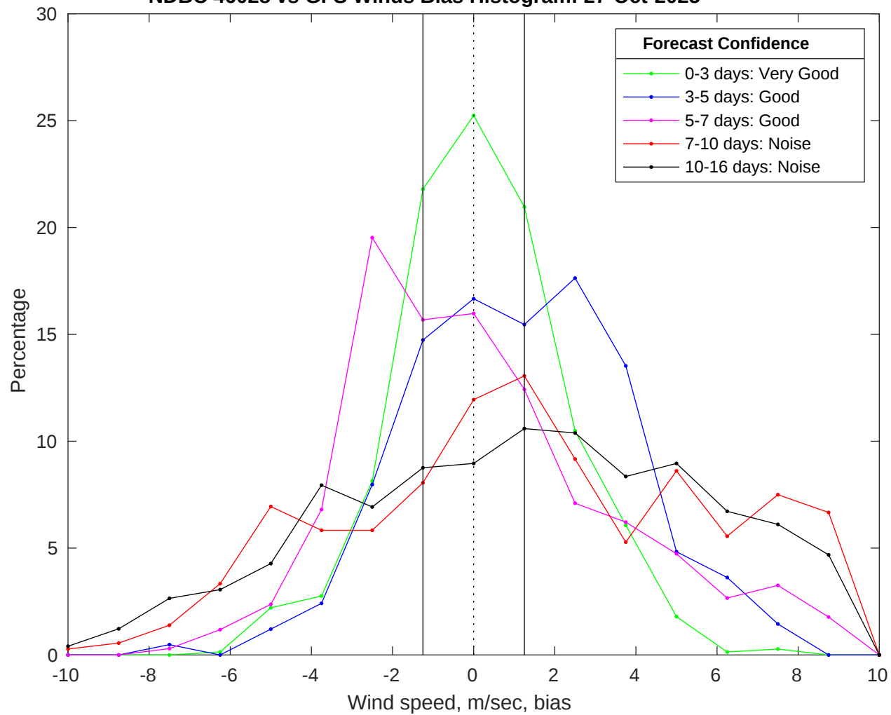
NDBC 46028 vs GFS Winds Bias Histogram: 27-Oct-2025
