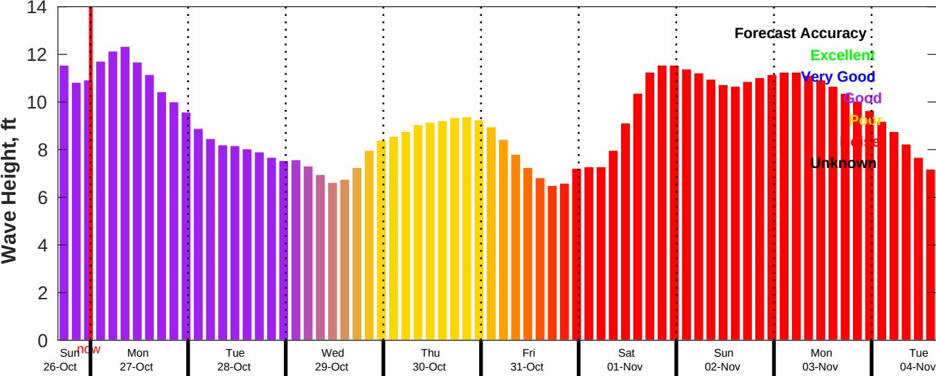
CMEMS Wave Forecast for NDBC 46028 from 26-Oct-2025 16:00:00 to 04-Nov-2025 16:00:00
