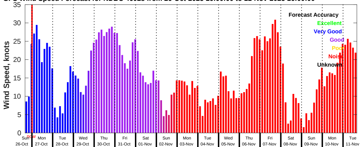
GFS Wind Speed Forecast for NDBC 46028 from 26-Oct-2025 16:00:00 to 11-Nov-2025 16:00:00
