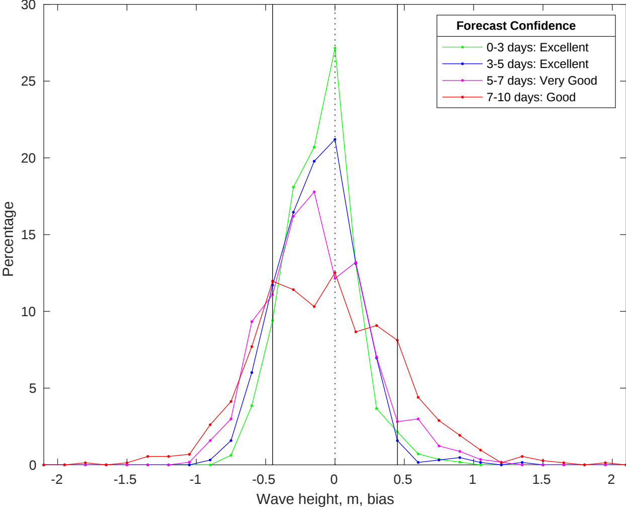
NDBC 46054 vs CMEMS Waves Bias Histogram: 27-Oct-2025
