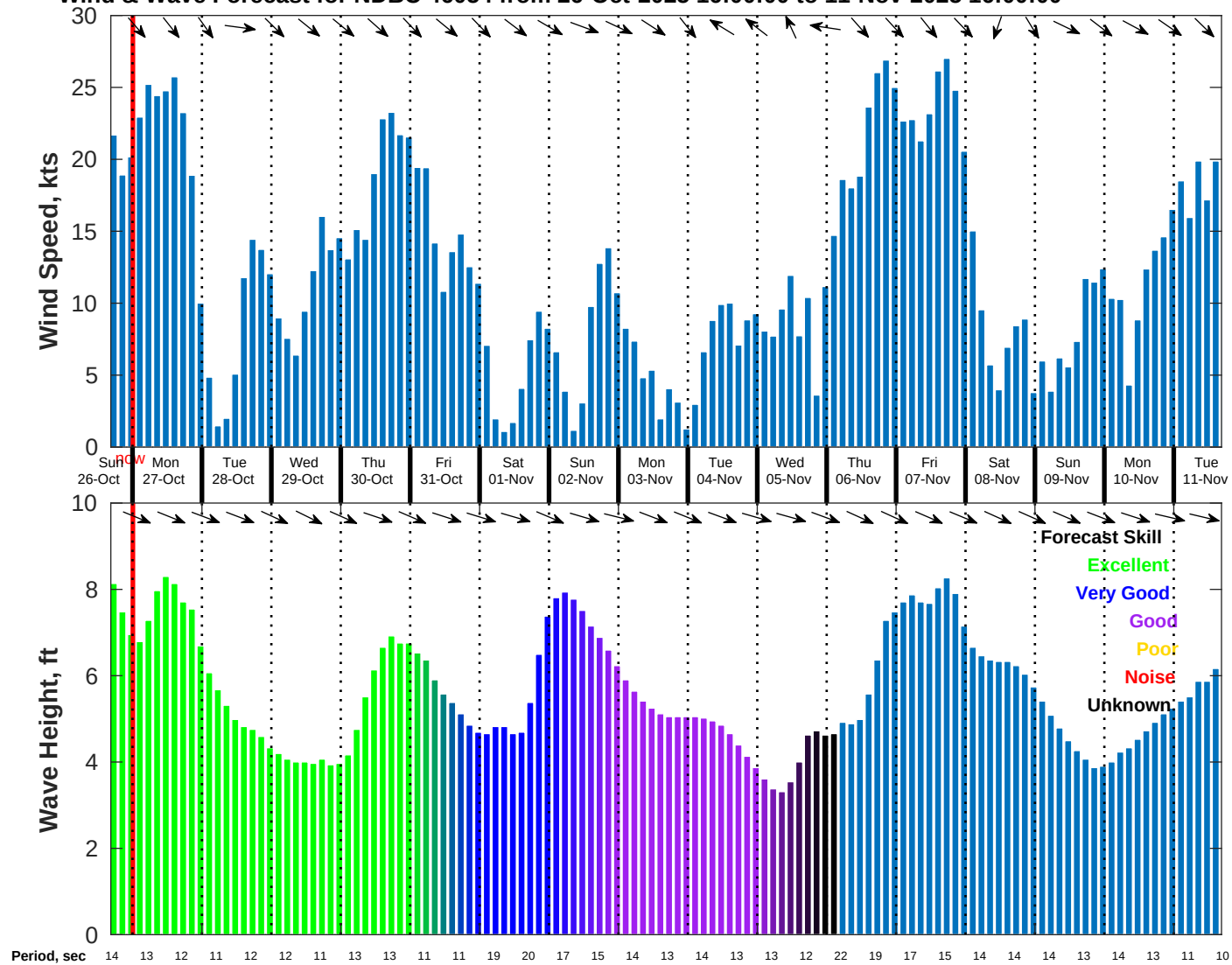
Wind & Wave Forecast for NDBC 46054 from 26-Oct-2025 16:00:00 to 11-Nov-2025 16:00:00
