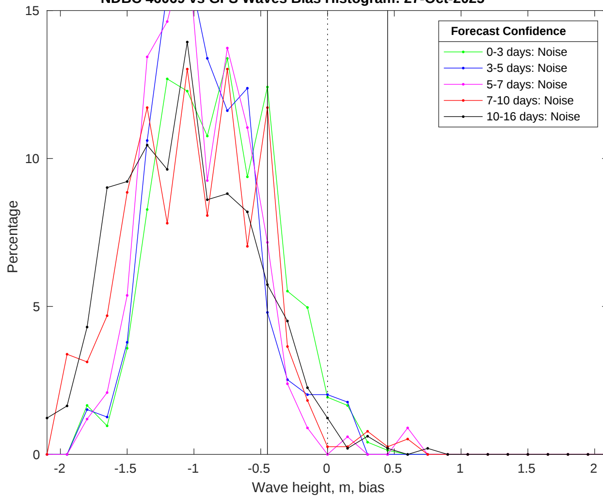
NDBC 46069 vs GFS Waves Bias Histogram: 27-Oct-2025
