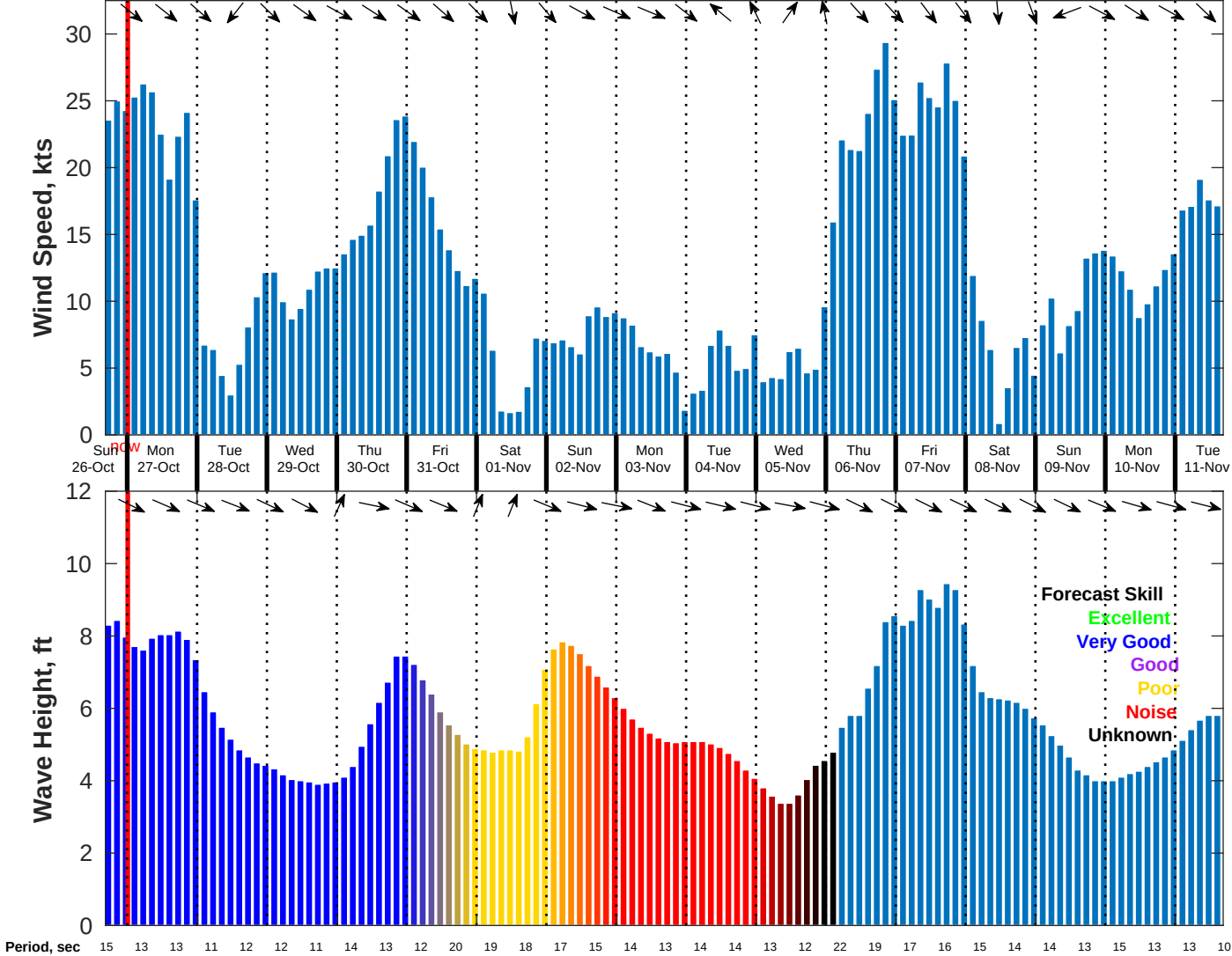
Wind & Wave Forecast for NDBC 46069 from 26-Oct-2025 16:00:00 to 11-Nov-2025 16:00:00
