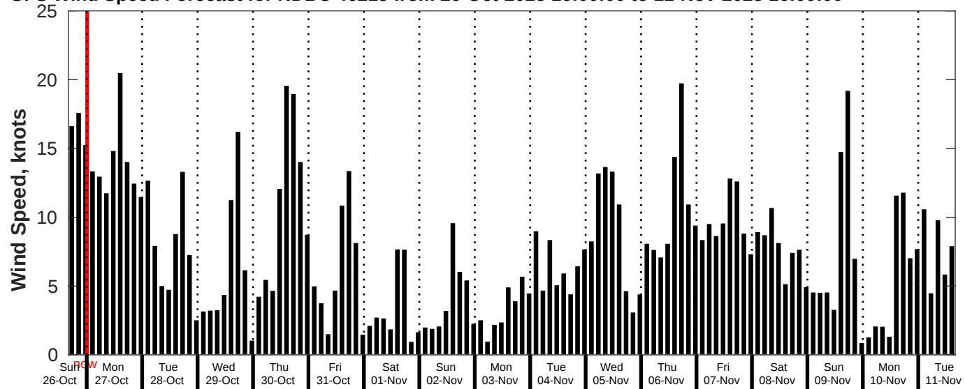
GFS Wind Speed Forecast for NDBC 46215 from 26-Oct-2025 16:00:00 to 11-Nov-2025 16:00:00
