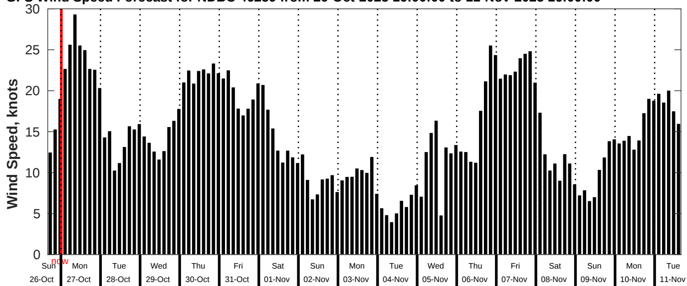
GFS Wind Speed Forecast for NDBC 46259 from 26-Oct-2025 16:00:00 to 11-Nov-2025 16:00:00
