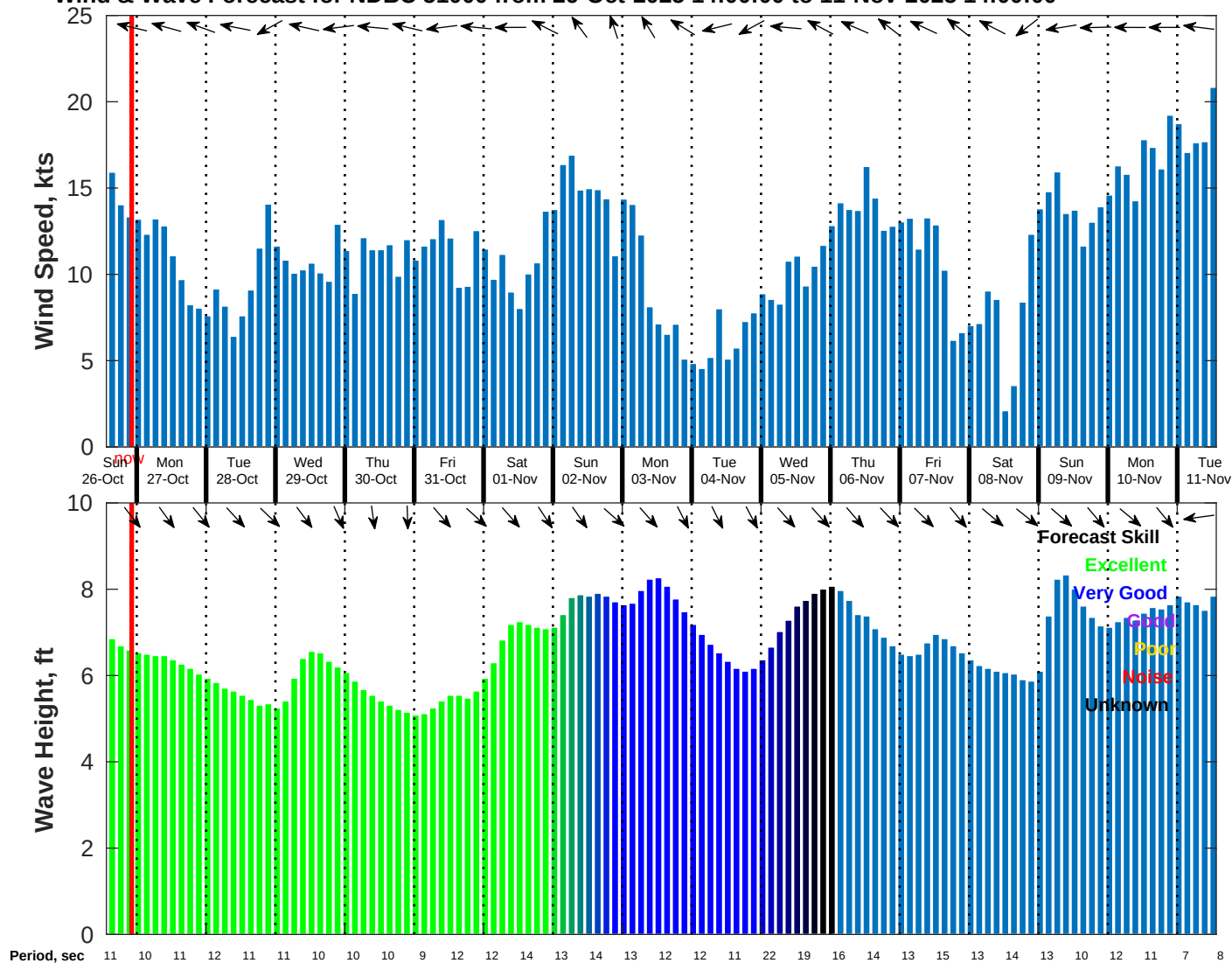
Wind & Wave Forecast for NDBC 51000 from 26-Oct-2025 14:00:00 to 11-Nov-2025 14:00:00
