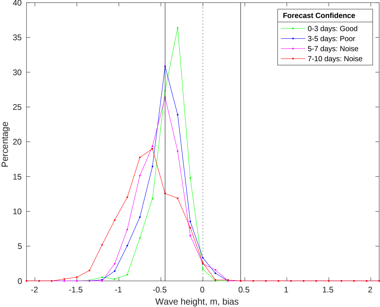
NDBC 51209 vs CMEMS Waves Bias Histogram: 27-Oct-2025
