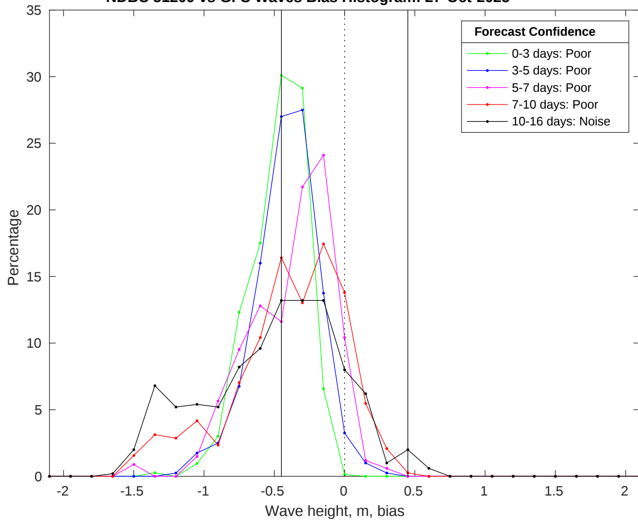
NDBC 51209 vs GFS Waves Bias Histogram: 27-Oct-2025
