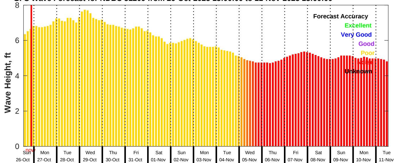
GFS Wave Forecast for NDBC 51209 from 26-Oct-2025 13:00:00 to 11-Nov-2025 13:00:00
