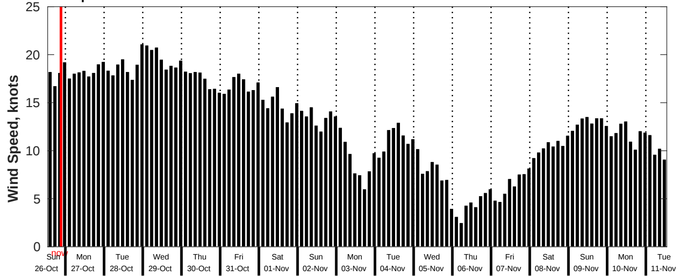
GFS Wind Speed Forecast for NDBC 51209 from 26-Oct-2025 13:00:00 to 11-Nov-2025 13:00:00
