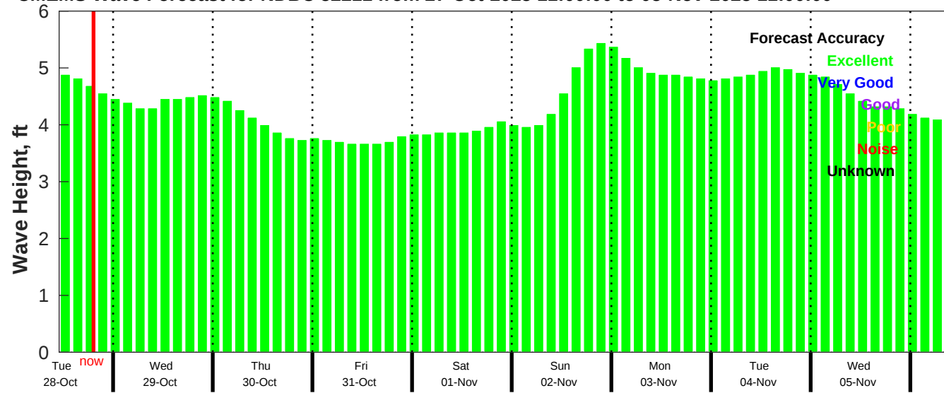
CMEMS Wave Forecast for NDBC 52211 from 27-Oct-2025 11:00:00 to 05-Nov-2025 11:00:00
