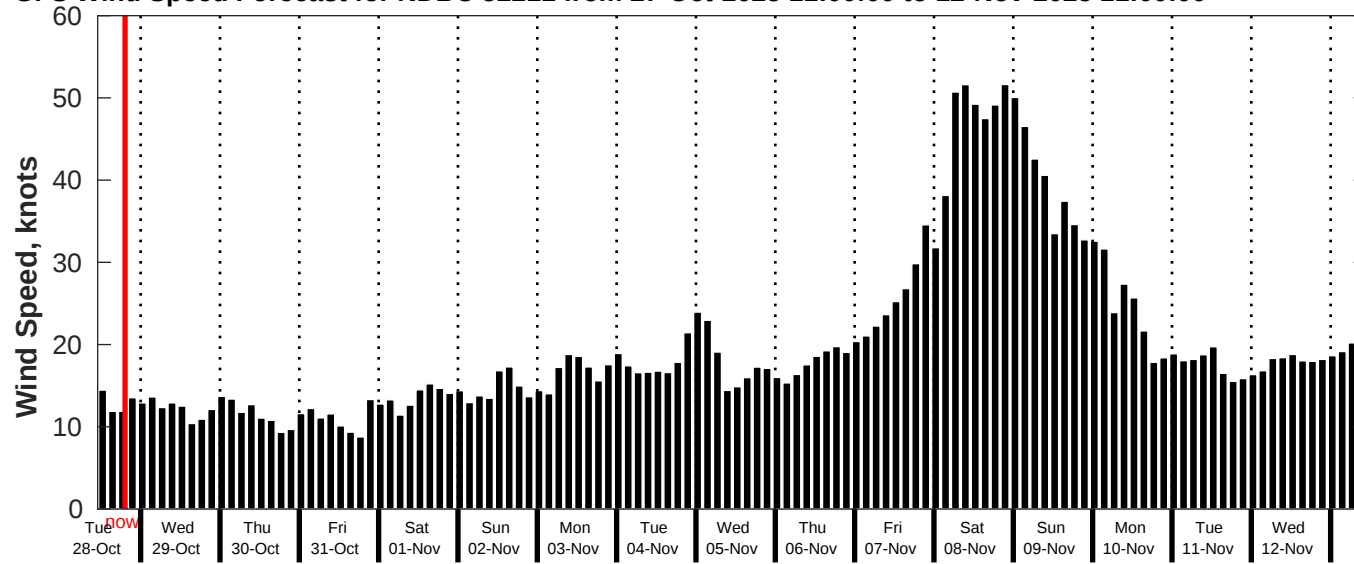
GFS Wind Speed Forecast for NDBC 52211 from 27-Oct-2025 11:00:00 to 12-Nov-2025 11:00:00
