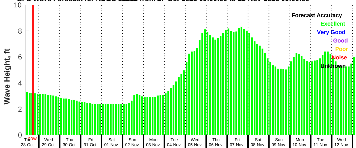
GFS Wave Forecast for NDBC 52212 from 27-Oct-2025 09:00:00 to 12-Nov-2025 09:00:00
