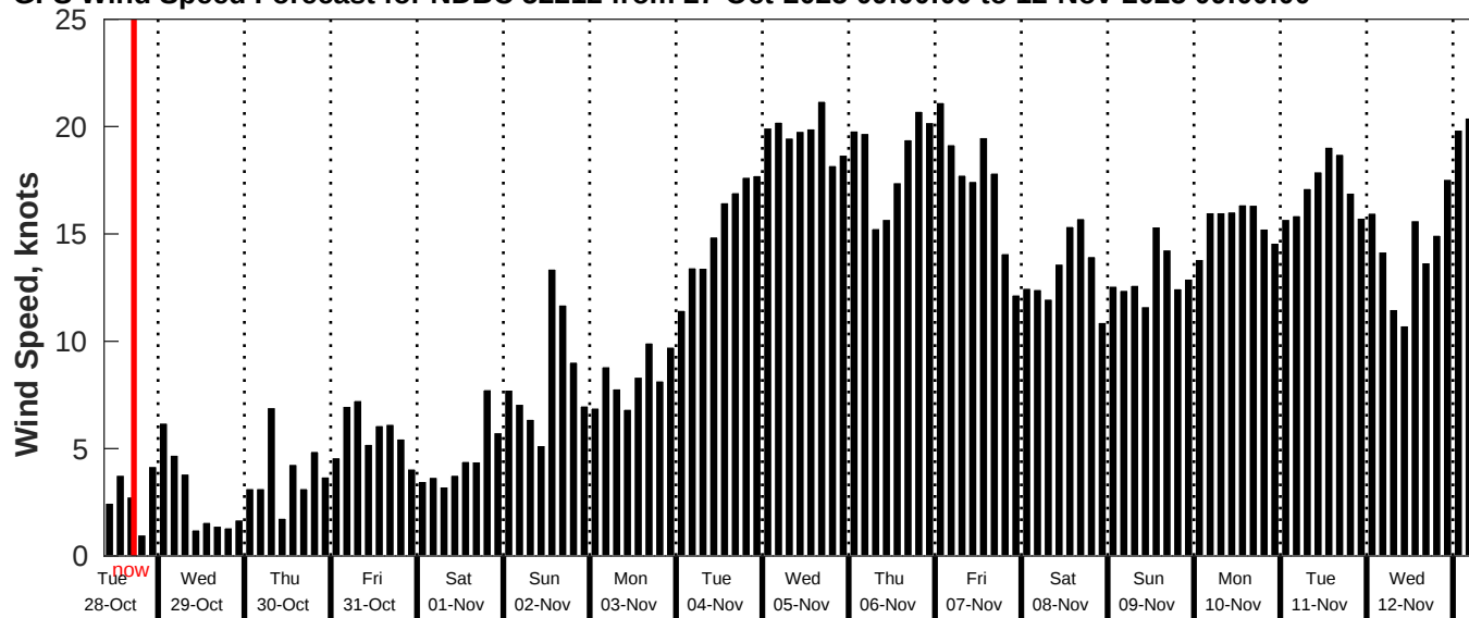
GFS Wind Speed Forecast for NDBC 52212 from 27-Oct-2025 09:00:00 to 12-Nov-2025 09:00:00
