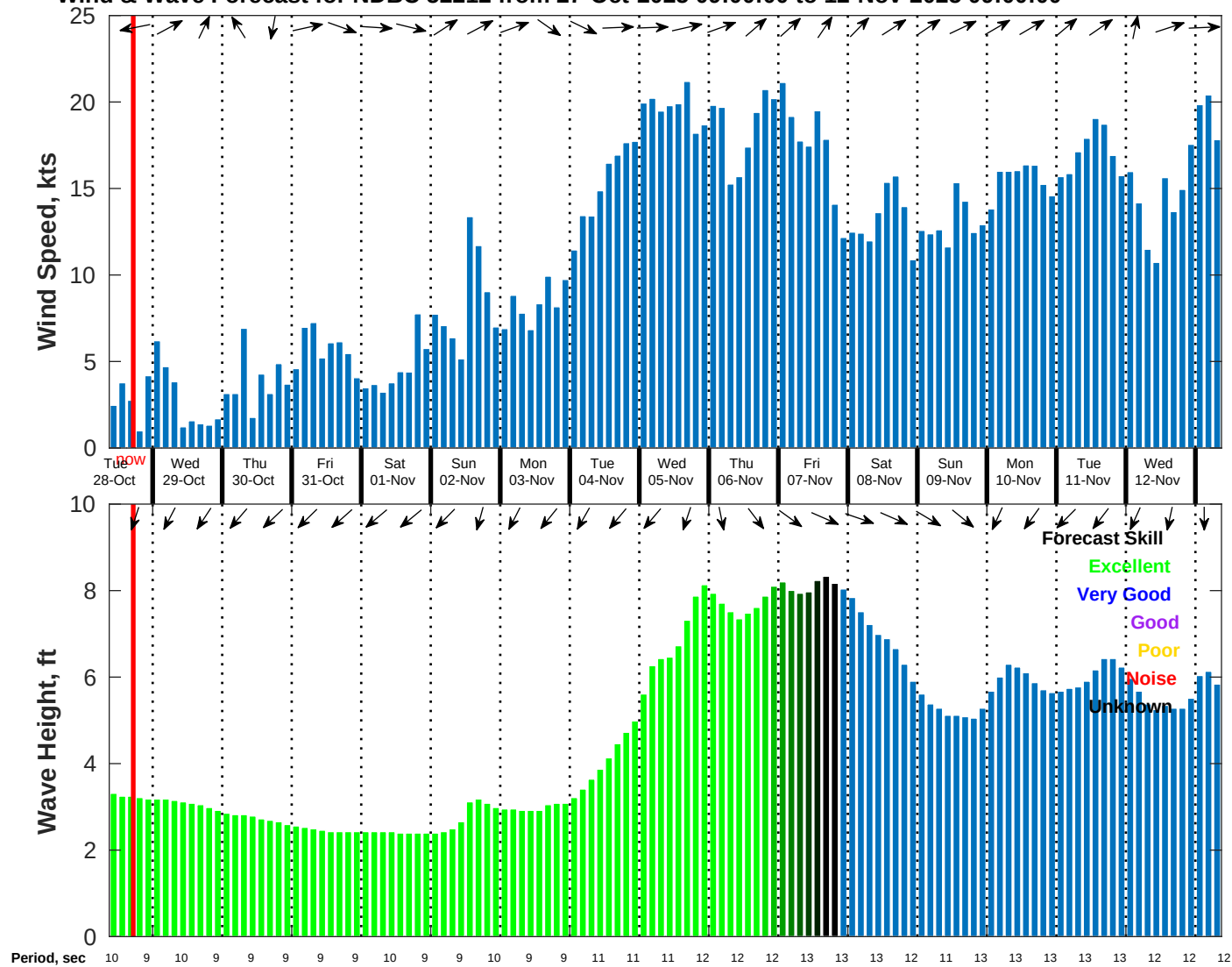
Wind & Wave Forecast for NDBC 52212 from 27-Oct-2025 09:00:00 to 12-Nov-2025 09:00:00
