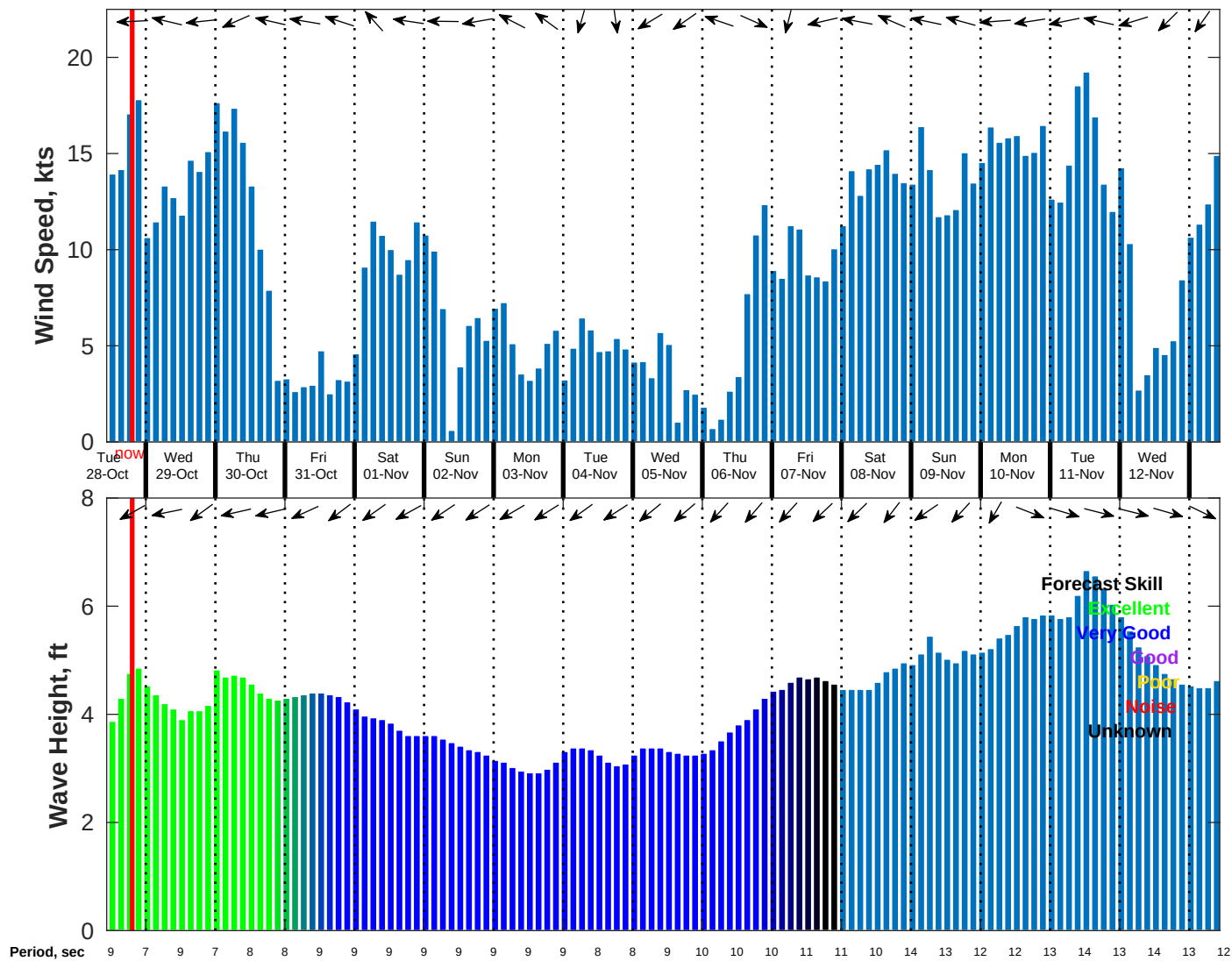
Wind & Wave Forecast for NDBC 52213 from 27-Oct-2025 11:00:00 to 12-Nov-2025 11:00:00
