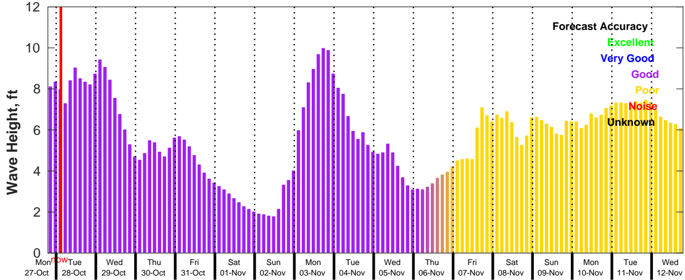
GFS Wave Forecast for NDBC 41004 from 27-Oct-2025 19:00:00 to 12-Nov-2025 19:00:00
