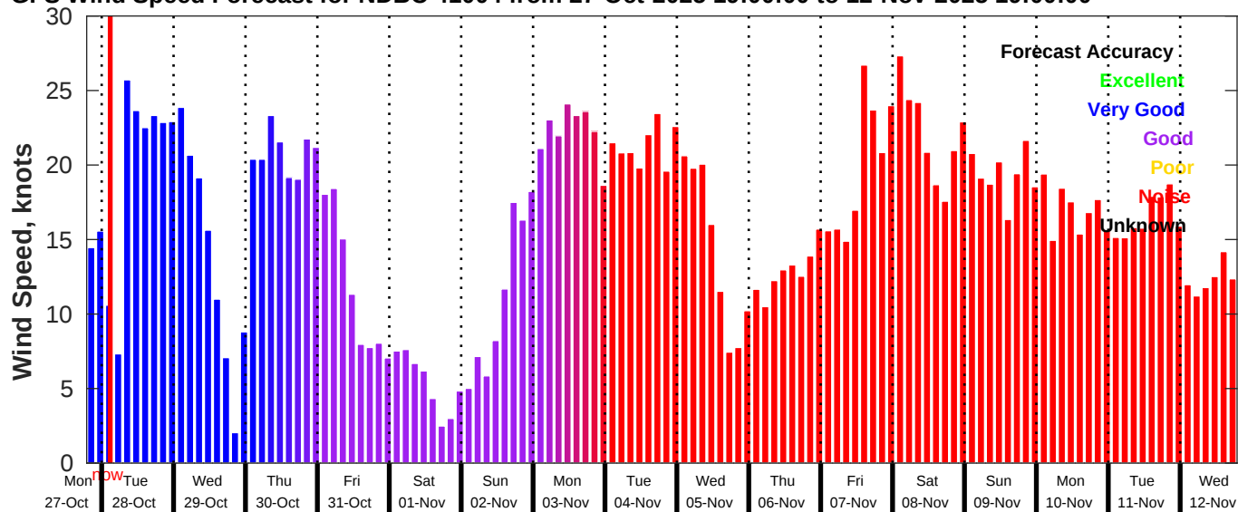
GFS Wind Speed Forecast for NDBC 41004 from 27-Oct-2025 19:00:00 to 12-Nov-2025 19:00:00
