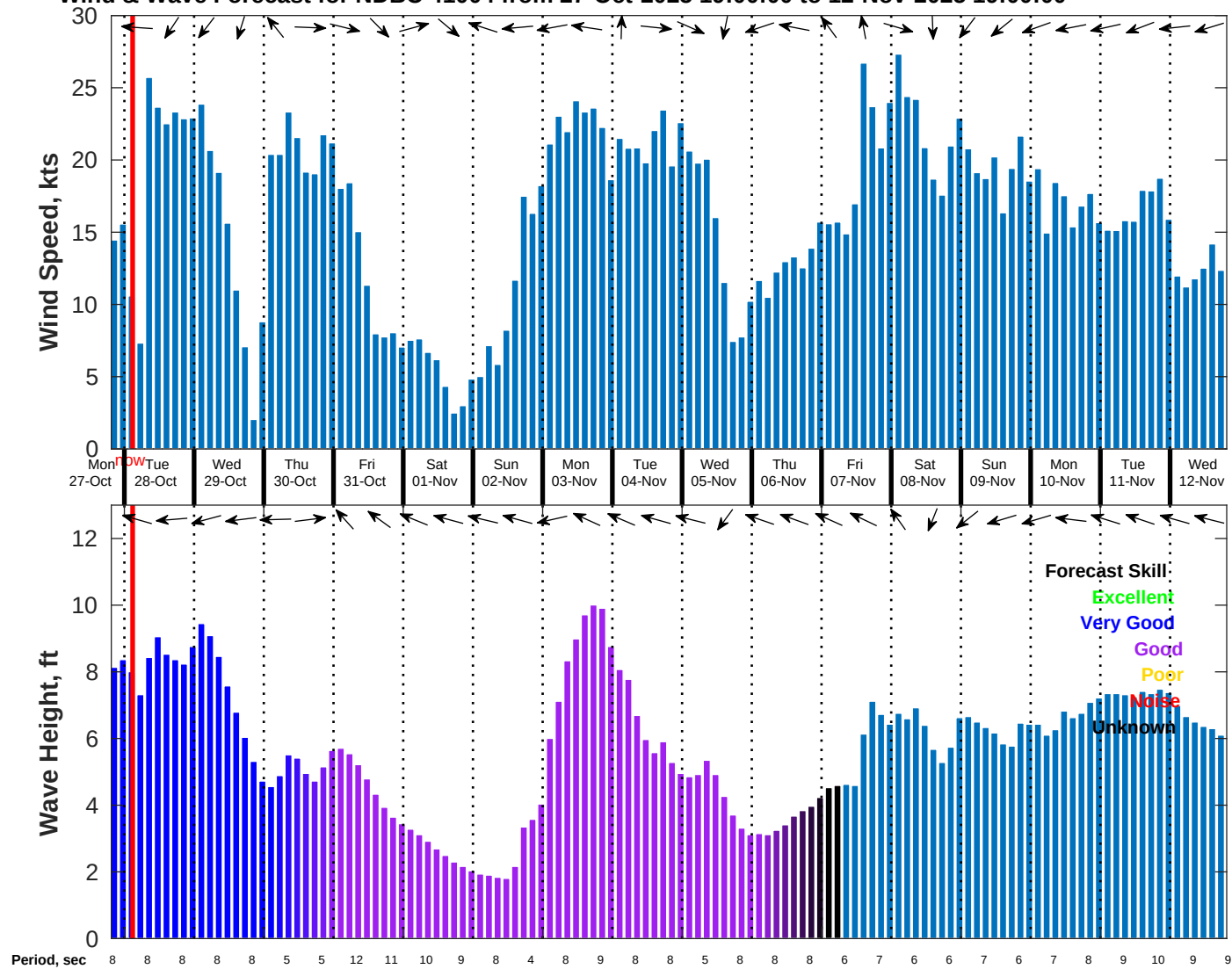
Wind & Wave Forecast for NDBC 41004 from 27-Oct-2025 19:00:00 to 12-Nov-2025 19:00:00
