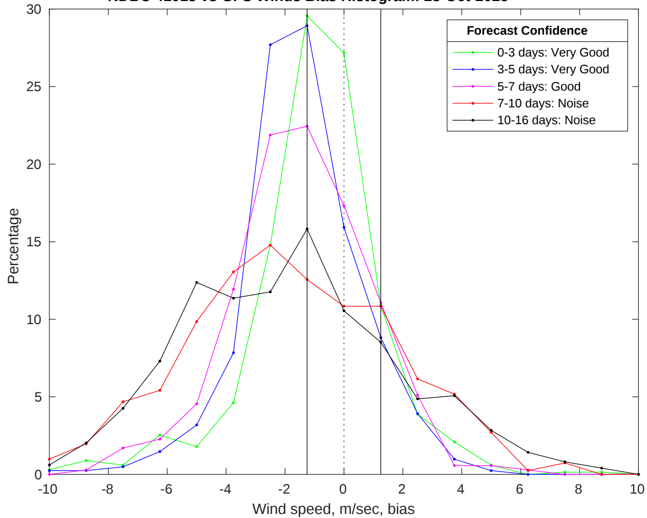
NDBC 41013 vs GFS Winds Bias Histogram: 28-Oct-2025
