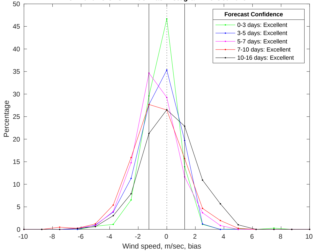
NDBC 41040 vs GFS Winds Bias Histogram: 28-Oct-2025
