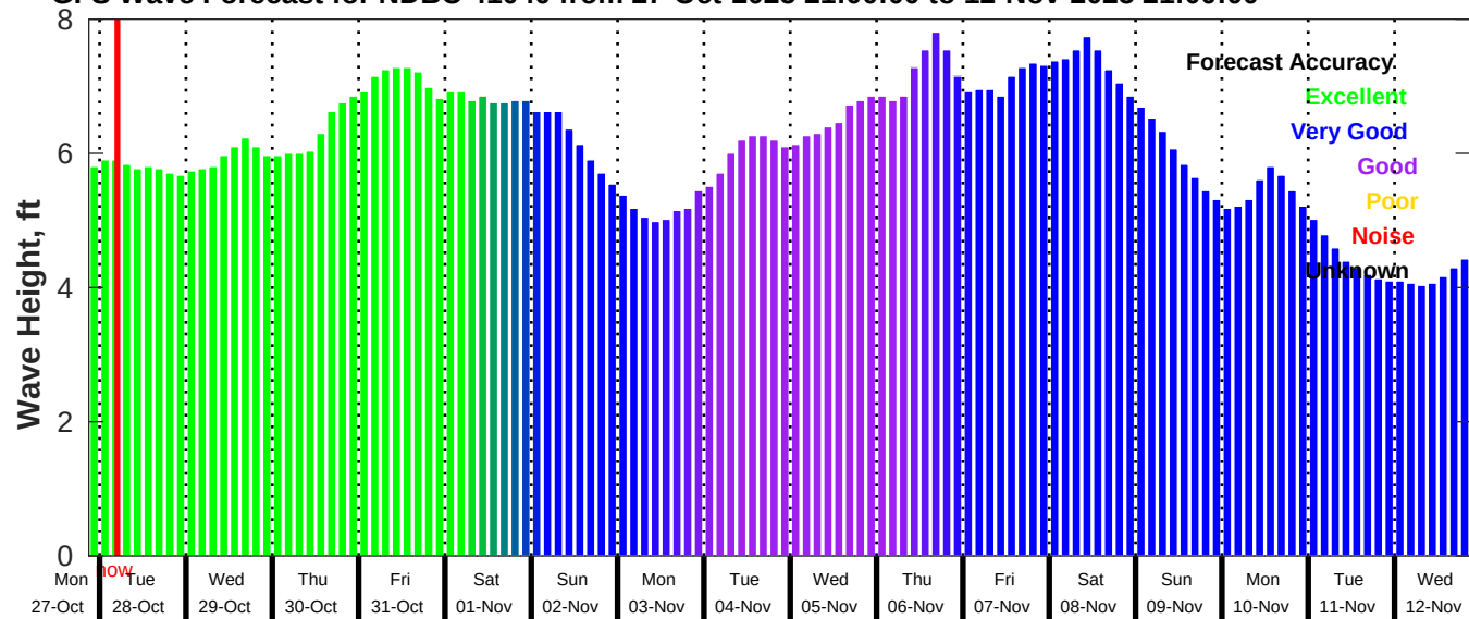
GFS Wave Forecast for NDBC 41040 from 27-Oct-2025 21:00:00 to 12-Nov-2025 21:00:00
