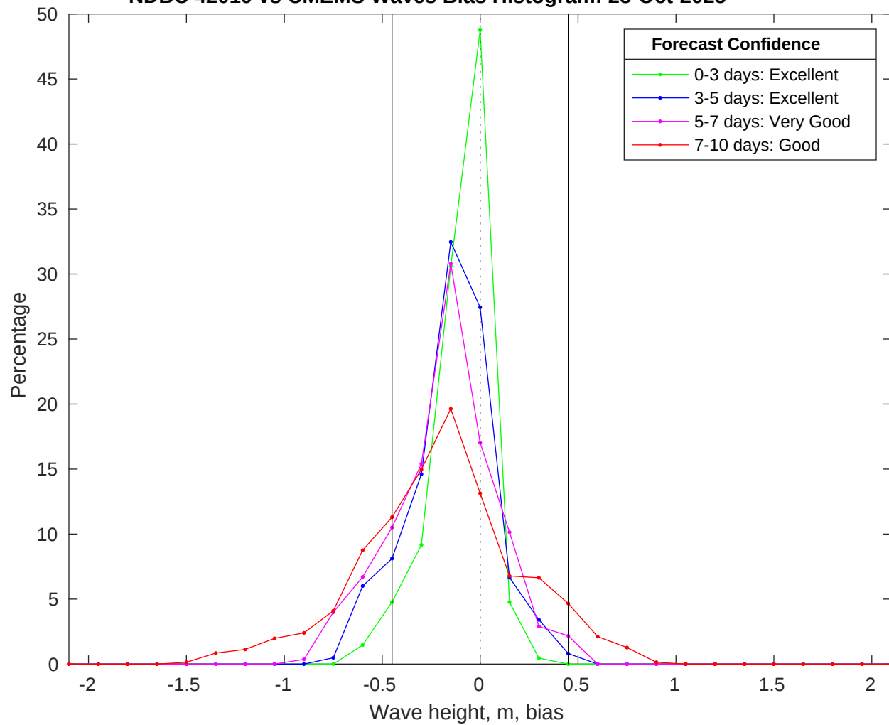
NDBC 42019 vs CMEMS Waves Bias Histogram: 28-Oct-2025
