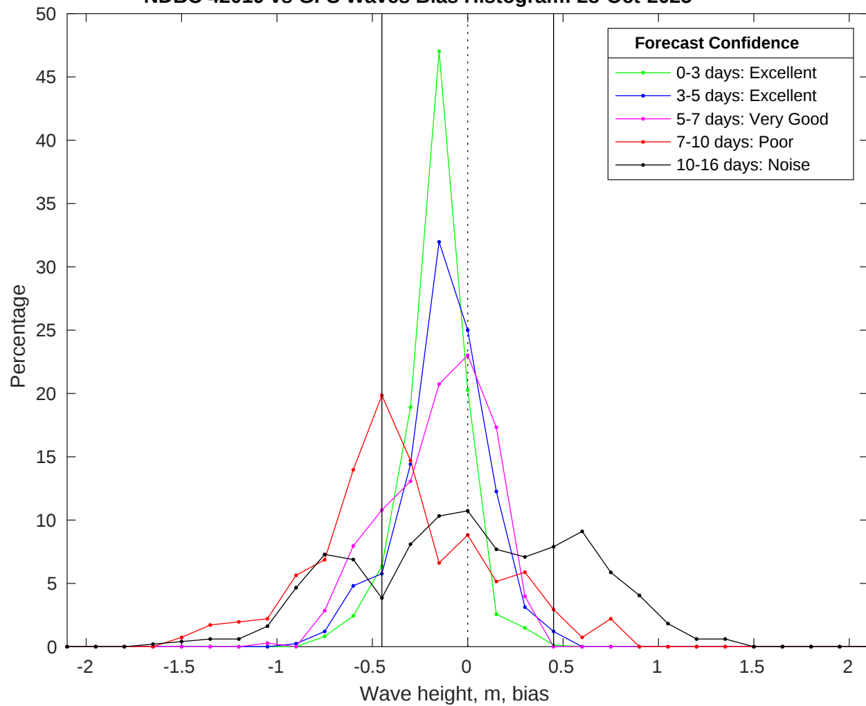
NDBC 42019 vs GFS Waves Bias Histogram: 28-Oct-2025
